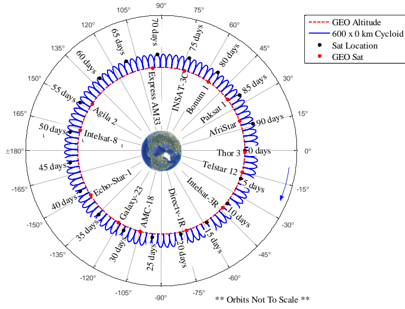
Figure 1 Carrier and GSO orbits in an Earth Centered Earth Fixed (ECEF) reference frame. Top - Carrier orbit in a co-planar, co-circular orbit, 300 km above GEO. Bottom - Carrier in a cycloid orbit with apogee 600 km above GEO and perigee at GEO altitude. The black dots represent the position of the carrier satellite as a function of time. The red dots are fixed GSO locations. The red dotted line is the geostationary orbit. The blue line is the orbit of the Carrier in an Earth Centered Earth Fixed (non-inertial) reference frame. The figure shows that it takes about 94 days for the carrier to return to the same GEO longitude.
